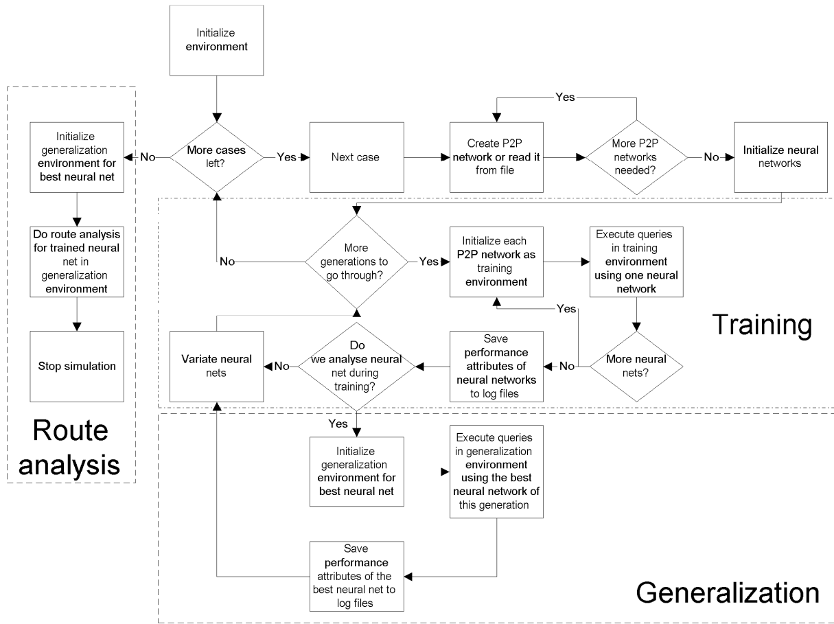
Figure 1. Execution Loops of P2PRealm
