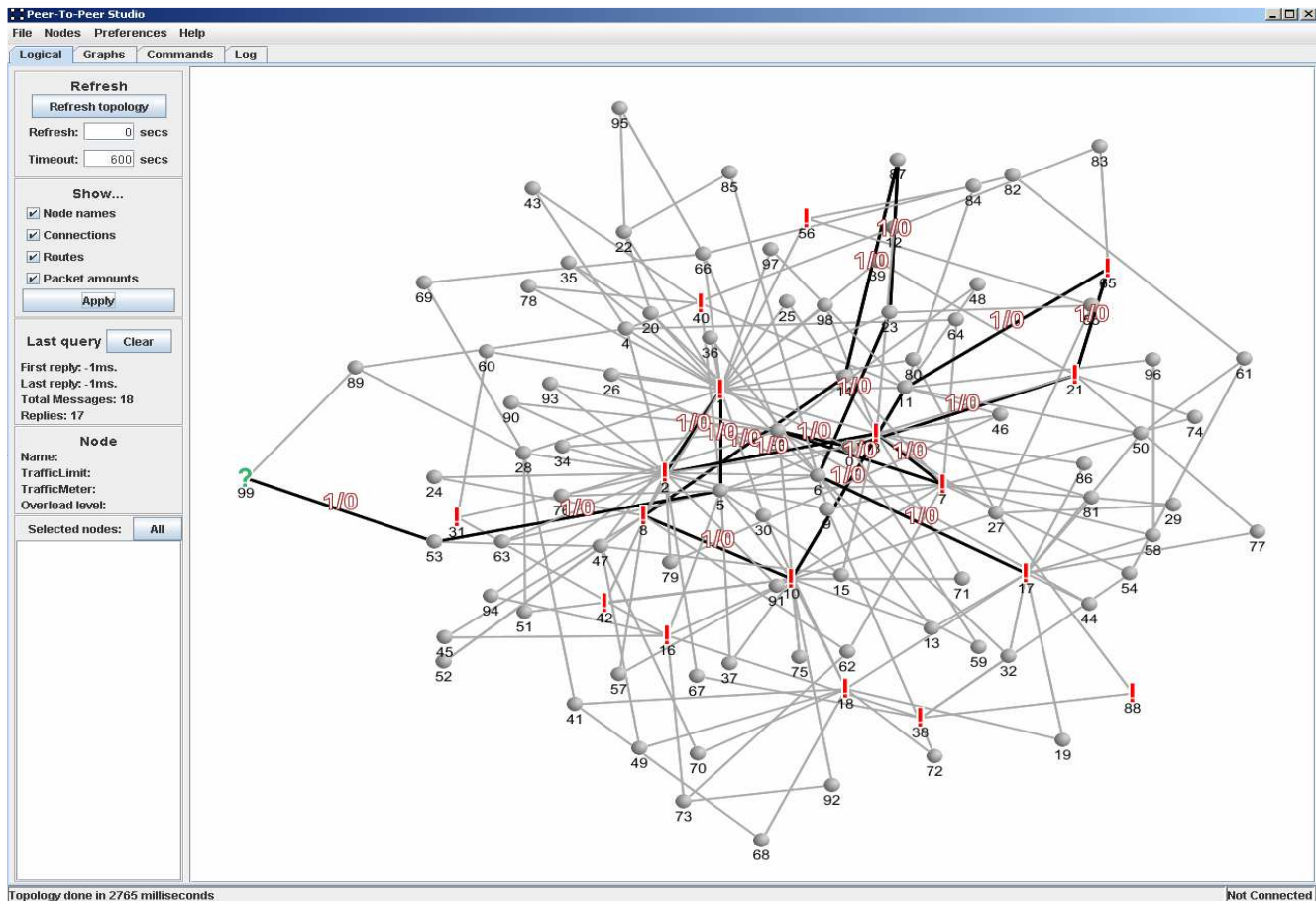
Figure 3. P2PStudio User Interface for P2PRealm
